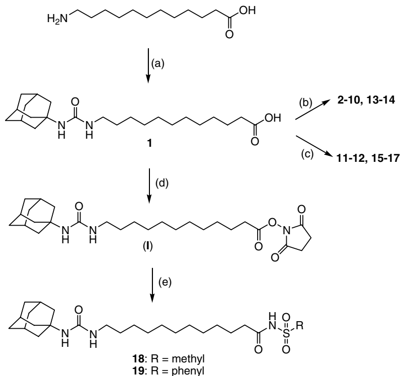
Scheme 1. Syntheses of alkyl ester ( 2–17 ) and sulfonamide ( 18 and 19 ) derivatives of 12-(3-adamantan-1-yl-ureido)dodecanoic acid. Reagents and conditions. (a) 1-adamantyl isocyanate, 1,2-dichloroethane, reflux; (b) alkyl bromide, \text{K}_2\text{CO}_3 , DMF, rt; (c) EDCI/DMAP or isobutyl chloroformate/triethylamine, corresponding alcohol or amine; (d) N -hydroxysuccinimide, 1,3-dicyclohexylcarbodiimide, THF, rt; (e) methanesulfonamide (for compound 18 ) or benzenesulfonamide (for compound 19 ), DMAP, HMPA, 90 °C.
