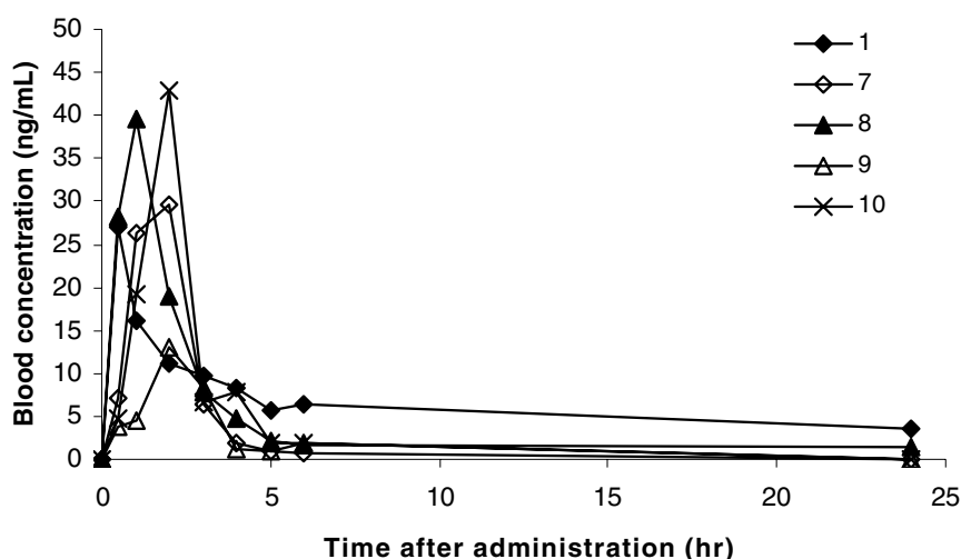
Figure 1. Blood concentration of AUDA 1 in mice as a function of time following oral gavage of sEH inhibitors 1 and 7–10 . All compounds were dissolved in olive oil and were given at 5 mg/kg body weight. Data are averages of results obtained from three different mice. Standard deviations were between 5% and 10%.
