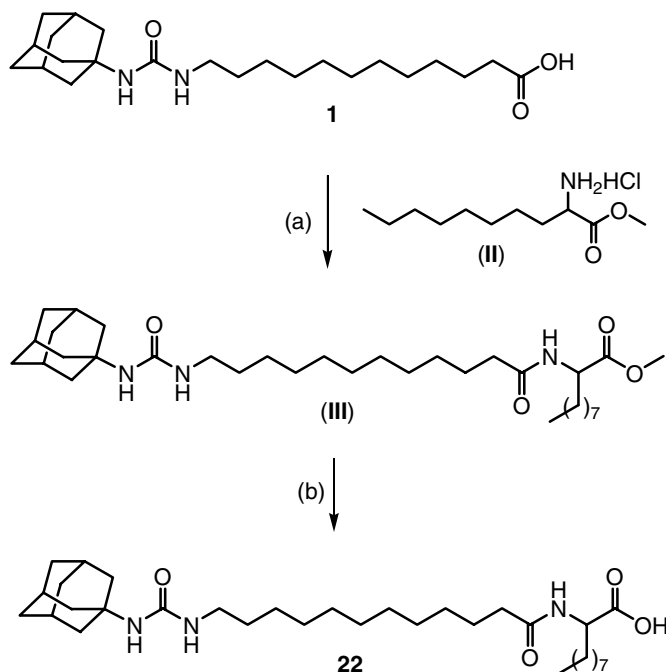
Scheme 2. Synthesis of 2-[12-(3-(adamantan-1-yl-ureido)dodecanoylamino]decanoic acid ( 22 ). Reagents and conditions: (a) 1—methyl 2-amino decanoate ( II ) was prepared from diethyl acetamido malonate and 1-bromooctane; 2— II , HBTU, DIEA, DMF, rt; (b) \text{LiOH}\cdot\text{H}_2\text{O} , DME, \text{H}_2\text{O} , rt.
